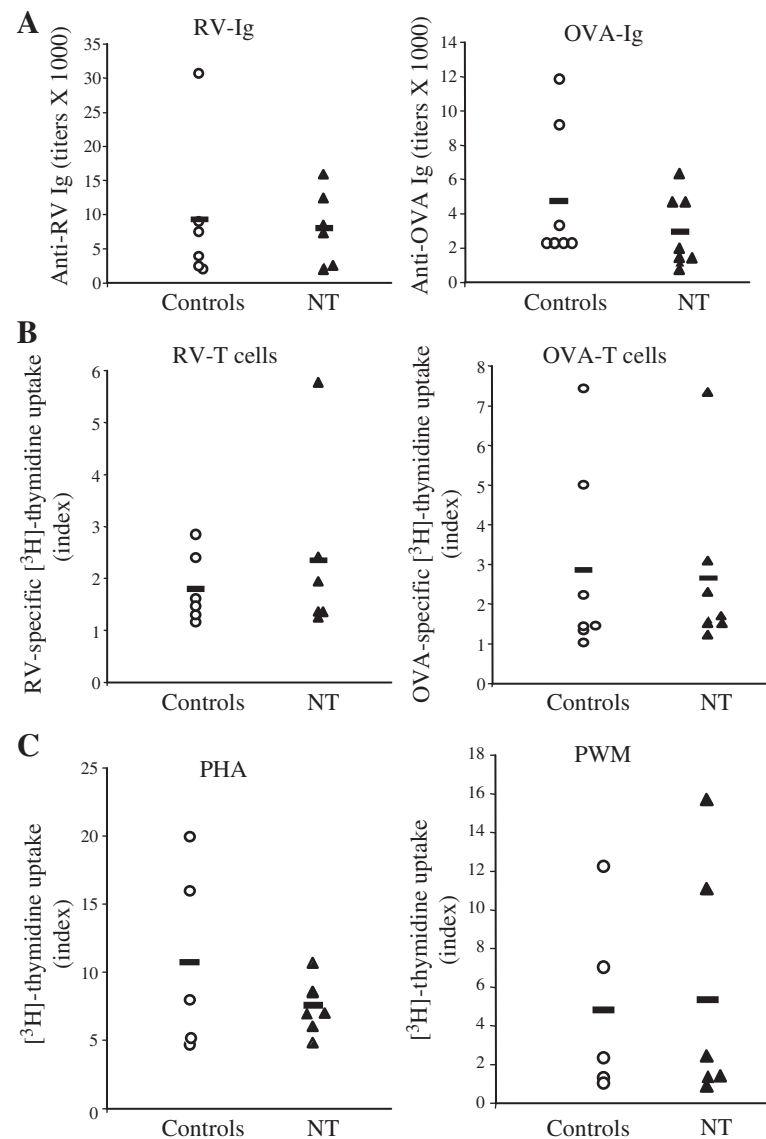
FIG. 3. Analysis of immune responses in control and SCNT cattle. Six control and SCNT cattle were vaccinated twice (D0 and D20) with inactivated bovine RV (RV group). Seven control and SCNT cattle, distinct from the RV group, were vaccinated twice (D0 and D20) with OVA (OVA group). (A) RV- and OVA-specific serum Ig were measured by ELISA on D30. No statistical difference was found between the control (empty circle) and SCNT (filled triangle) cattle ( p = 0.80 and 0.78 for RV and OVA, respectively). (B) PBMCs were collected on day 35 and restimulated in vitro with 3 mg/mL purified RV (RV group) or 500 mg/mL OVA (OVA group). [ ^3\text{H} ]-Thymidine incorporation was done on the last 18 h of a 5-day culture. Stimulation indexes are shown. No statistical difference was found between the control and SCNT cattle ( p = 0.23 and p = 0.48 for RV and OVA, respectively). (C) PBMCs were collected from five control and six SCNT cattle and they were stimulated in vitro with PHA (50 mg/mL) and PWM (10 mg/mL). [ ^3\text{H} ]-Thymidine incorporation was done on the last 18 h of a 48-h culture. Stimulation indexes are shown. No statistical difference was found between the control and SCNT cattle ( p = 0.16 and 0.43 for PHA and PWM, respectively).
