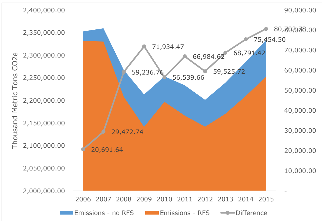
Figure 1: U.S. Transportation Fuel Mix Carbon Emissions Under Two Scenarios, 2006-2015
